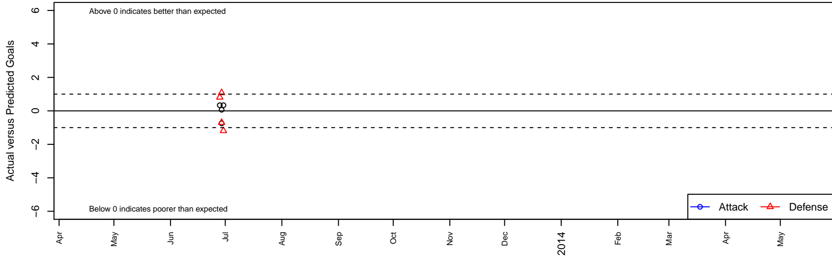
Crossfire Oregon B94 Dots are actual minus expected GF (blue circles) and GA (red triangles). Blue line is smoothed change in attack strength. Red is smoothed change in defense strength.
